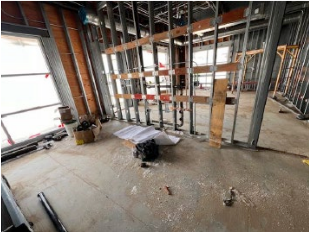
MEP Rough-In / Wood Blocking / Wall Framing
