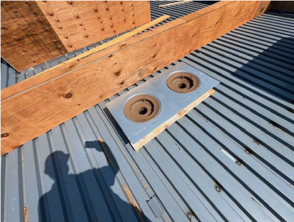
Metal deck, plywood sheathing & roof drains
